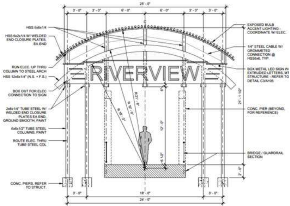
C1 BRIDGE SIGN - FRONT ELEV. 1/4" = 1'-0"
