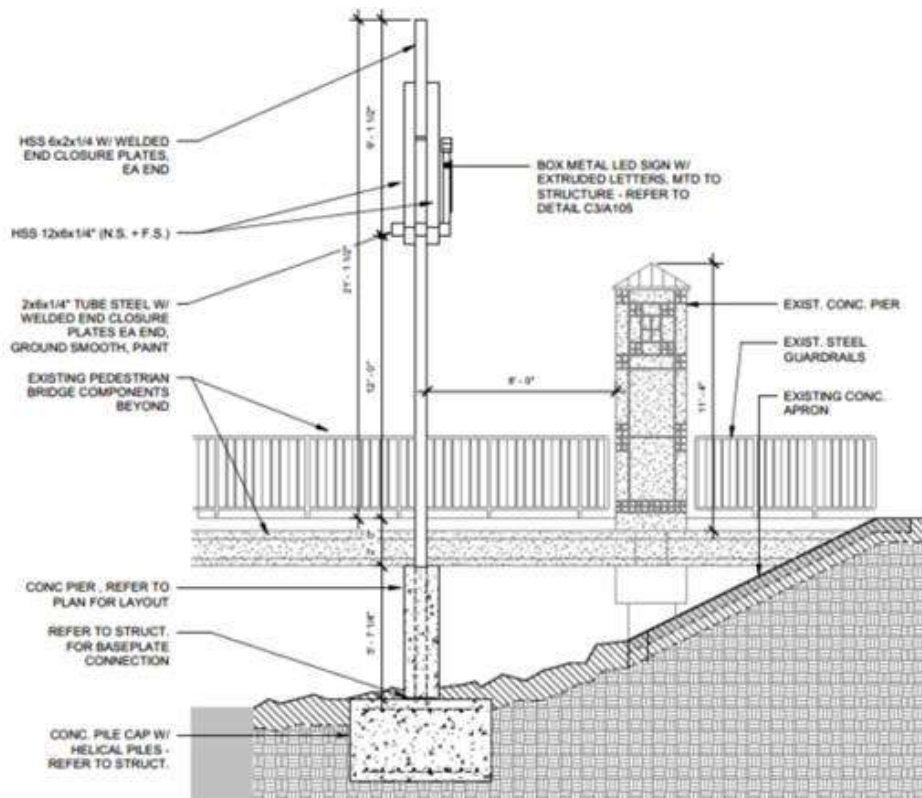
A2 BRIDGE SIGN - SIDE ELEV. 1/4" = 1'-0"
