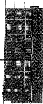
PROPOSED STUDENT APARTMENTS EAST ELEVATION
