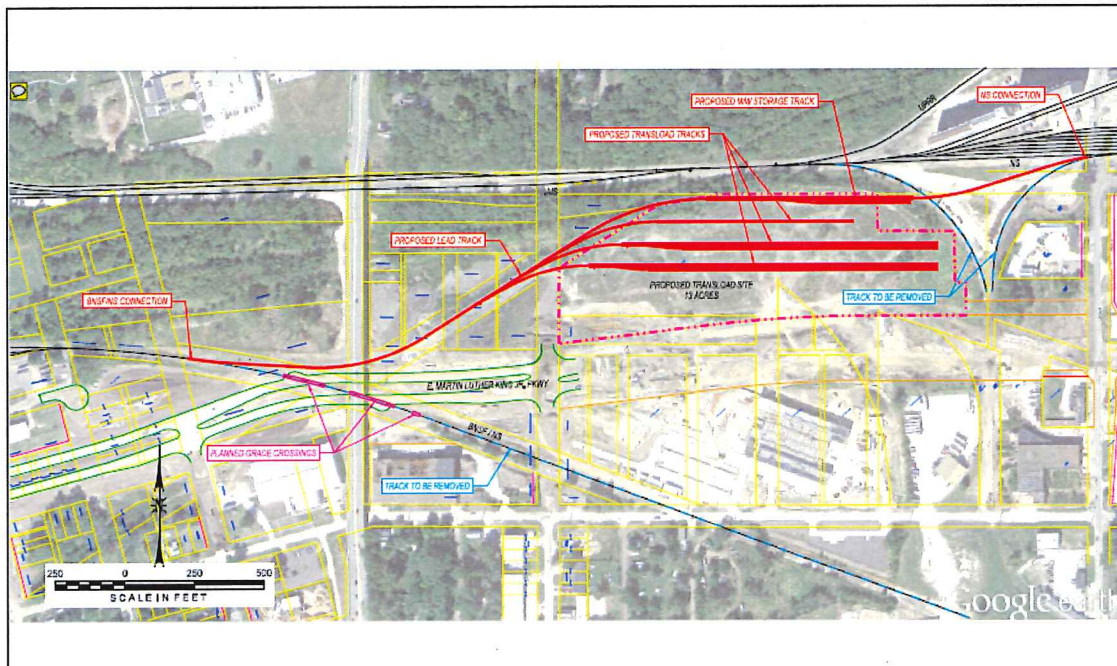
Figure 8 – Site Design
