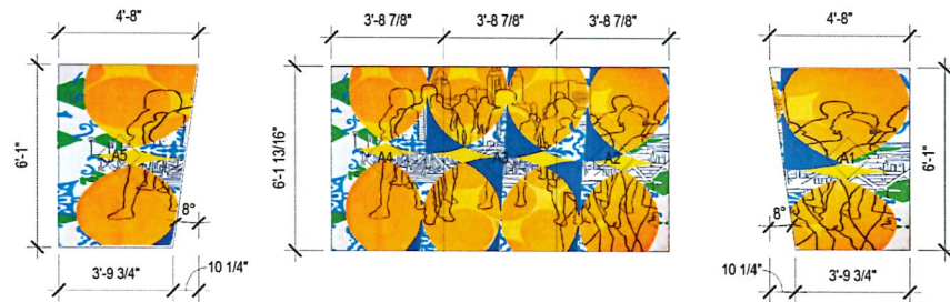
2 GLASS PANEL - ELEVATIONS SCALE: 1/4" = 1'-0", REF: A1 / A1.02
