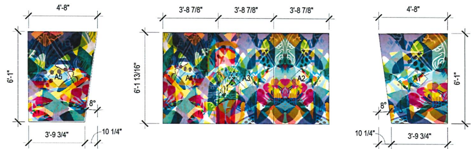
GLASS PANEL - ELEVATIONS SCALE: 1/4" = 1'-0", REF: A1 / A1.02
