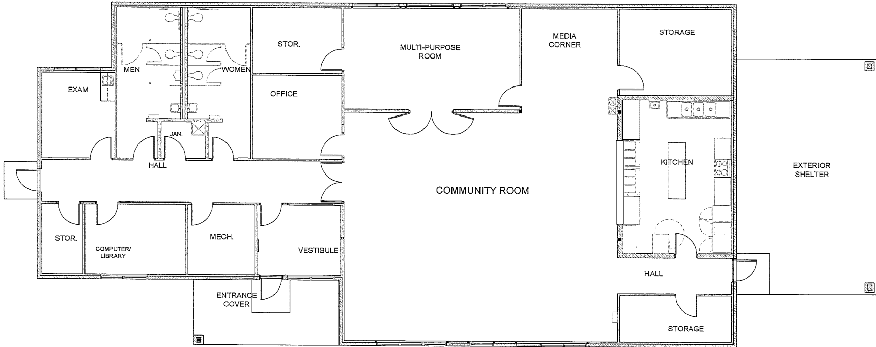
N PLAN MARTIN LUTHER KING JR. SHELTER
